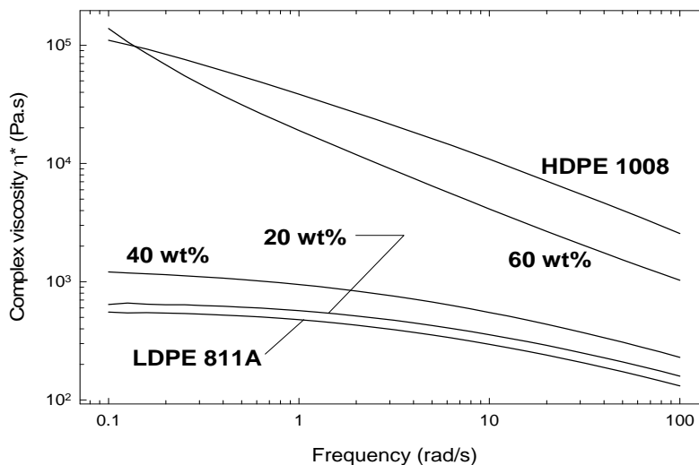
Chart 2: Complex Shear Viscosity as a Function of Frequency at 200°C
