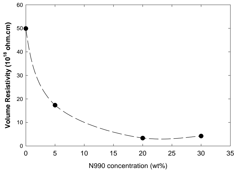
Chart 3: Volume Resistivity of Polyethylene/Thermax® N990 Compounds
