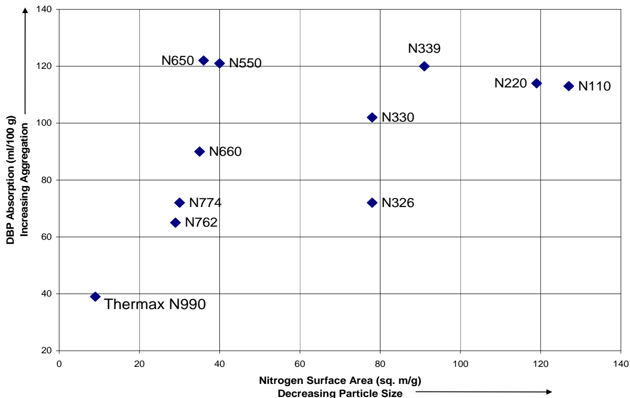
Chart 1: The Carbon Black Spectrum
